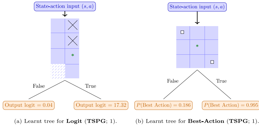
Fig. 14. Two trees with depth limits of d = 1 that were built for the game of Tic-Tac-Toe. A shaded square indicates that position must be an “off-board” position (i.e., not exist as a part of the board). A small white square indicates a position that must be empty.
