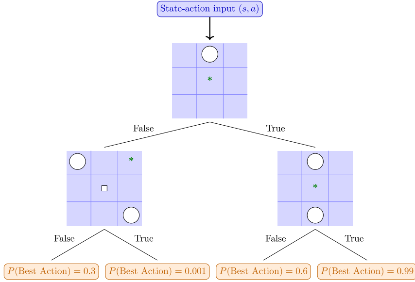
Fig. 8. Example best-action classification tree for a handcrafted Tic-Tac-Toe policy, modelled as a binary classification tree that takes state-action pairs (s, a) as inputs, and produces probability estimates of a being a “best action” in s as outputs.
