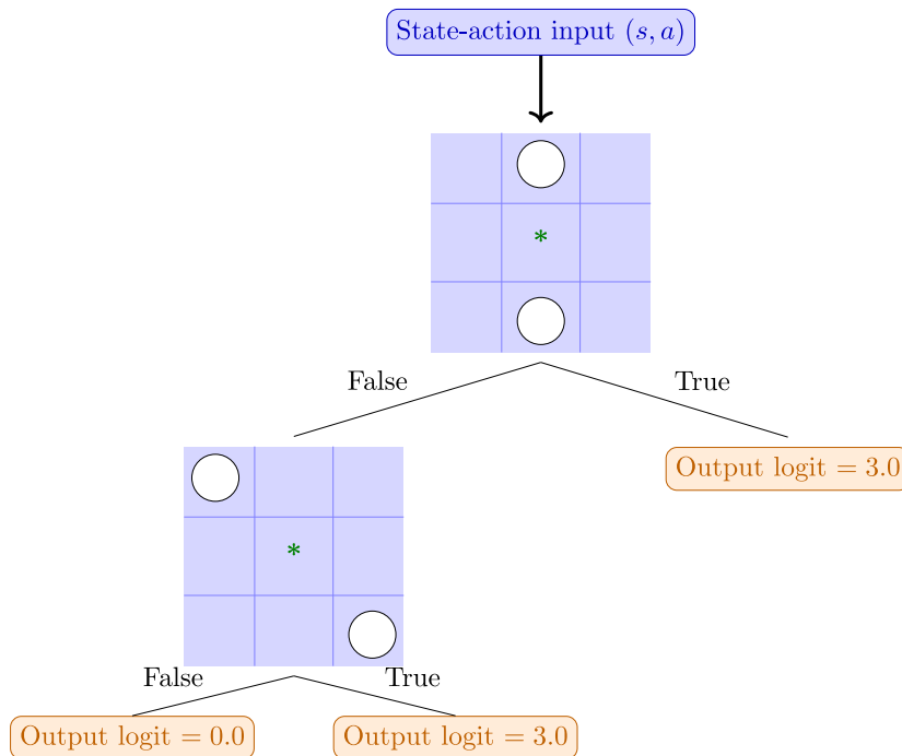
Fig. 6. Example logit regression tree for a handcrafted policy for Tic-Tac-Toe, modelled as a regression tree that takes state-action pairs (s, a) as inputs and produces a single logit for such a pair as output. This regression tree can detect actions that complete any (assuming local rotations and reflections of features are used, which we do) orthogonal or diagonal line by placing the third stone in the middle of such a line, and assigns logit values of 3.0 to such actions. Any other action is assigned a logit value of 0.0. These outputs are meaningless on their own, but in combination with logits for other legal actions can easily be transformed into probabilities by a computer program.
