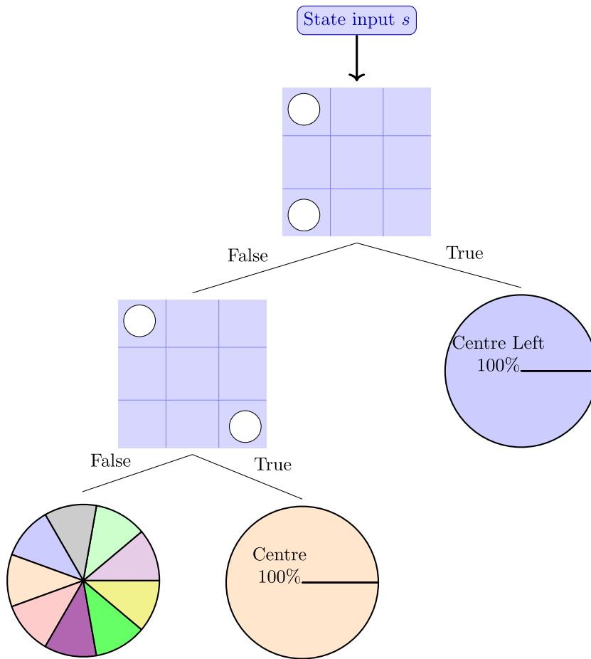
Fig. 5. Example of a handcrafted policy for Tic-Tac-Toe, modelled as a decision tree that takes states as inputs and produces probability distributions over all possible actions as outputs. This decision tree can recognise two particular cases of winning actions for the white player, but otherwise recommends a uniform distribution over all actions.
