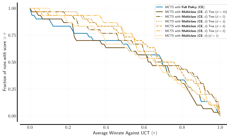
Fig. 13. Performance profiles summarising the performance of MCTS agents biased by several different policies against UCT, across 30 different games.
