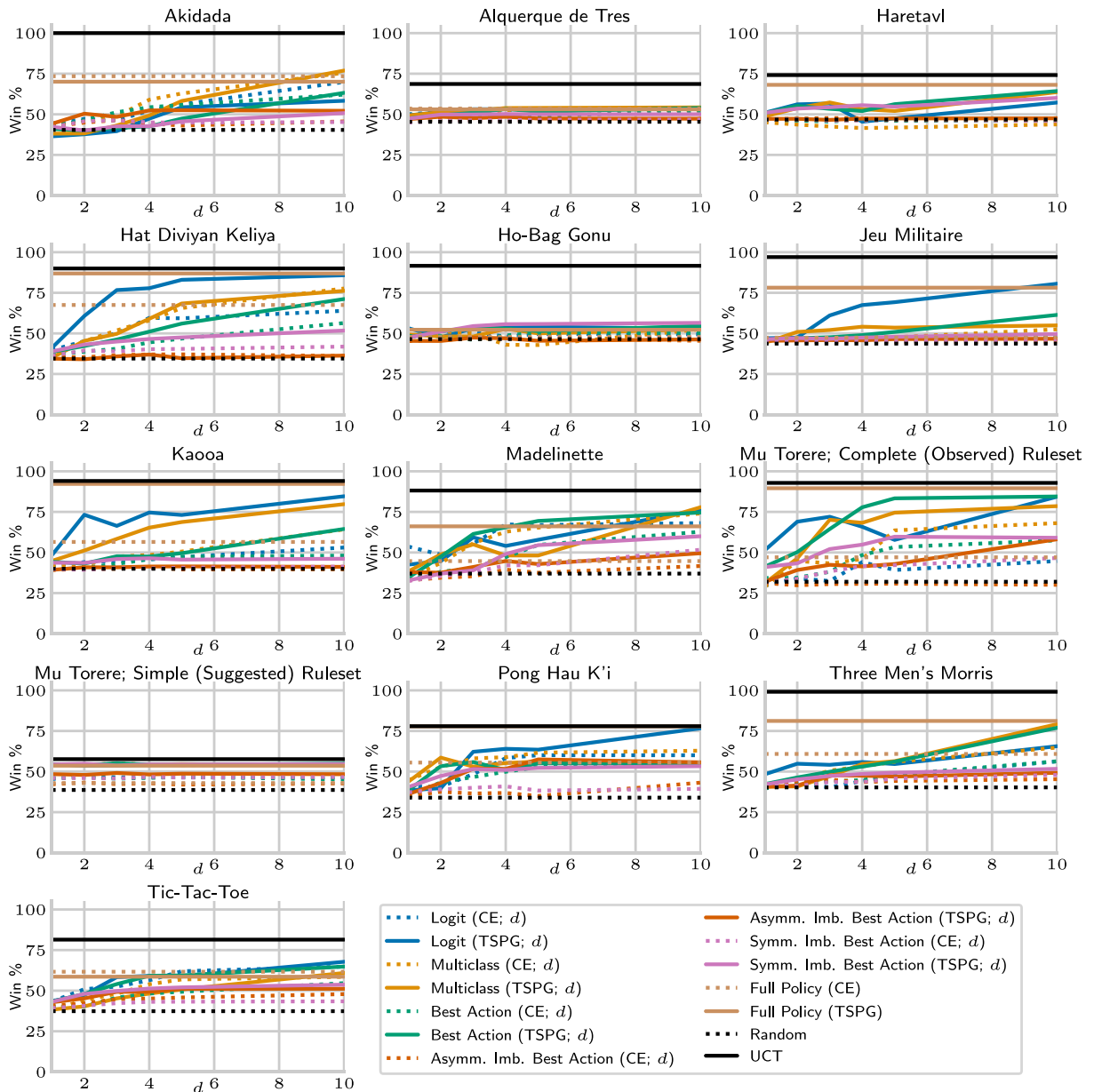
Fig. 9. Win percentages, averaged over all other agents as opponents, for various types of agents in 13 small games. Data plotted for maximum decision tree depths d \in \{1, 2, 3, 4, 5, 10\} along x -axis.
