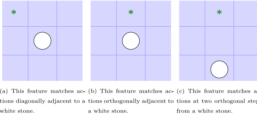
Fig. 4. MCTS-based players have a strong tendency to open games of Tic-Tac-Toe in the centre of the board. Therefore, it is highly likely for every action available in the first turn of the second player to match either the feature depicted in (a) or the one in (b). If the first player opens in a corner, the second player also has legal moves in their first turn that match the feature depicted in (c), but this is rarely observed in self-play between MCTS agents.
