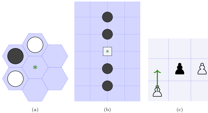
Fig. 1. Three examples of local state-action features that may be useful in various games. A small square indicates a position that must be empty. Uncovered sites are drawn for ease of interpretation, but play no role in the feature; they may be empty or non-empty or even not exist at all. (a) This feature matches actions that either complete or break a “bridge” of white pieces, depending on which player is the player to move. (b) This feature matches actions that either complete or break a line of five black pieces. (c) This feature matches actions that move the bottom-left white pawn in such a way that the black pawn becomes flanked by two white pawns.
