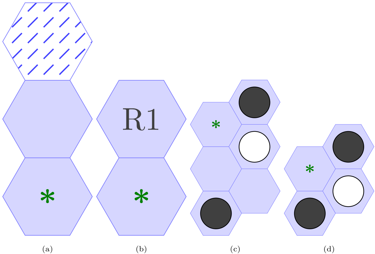
Fig. 15. Four features for the first player (white) in the game of Hex. (a) The first feature selected by Logit (TSPG; d ) trees. It matches any move in the second ring of cells from the edge of the board. (b) The first feature selected by Multiclass (TSPG; d ) trees. It matches any move that has an adjacent position which is closer to the region with index 1 (which, in Ludii, is the set of all cells along the black edges, which the black player aims to connect) than the position of the move. In practice, this feature applies to any move except for moves along the black board edges. (c) The first feature selected by Best-Action (TSPG; d ) trees, including imbalanced variants. Note that the undecorated cells are unrestricted; they need not be empty. (d) A bridge intrusion feature, which is a well-known tactic for Hex to stop the two black stones from connecting.
