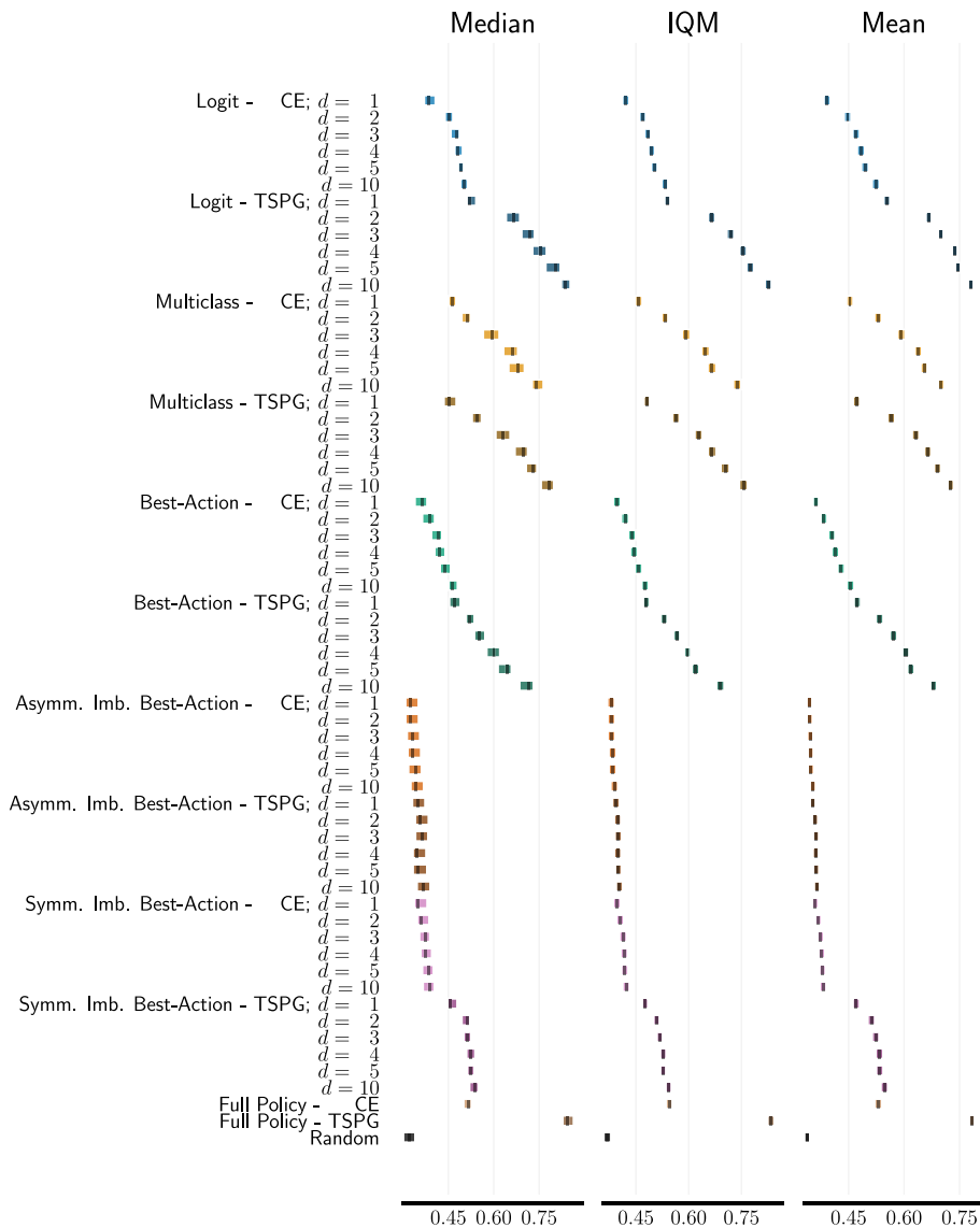
Fig. 11. Aggregate metrics for the performance levels of all 63 agents in the set of 30 games. The median, interquartile mean (IQM), and mean of the win rates are computed over runs in all games against all possible opponents. Coloured bars represent 95% bootstrap confidence intervals, estimated from 10,000 bootstrap replicates using the rliable library [43].
