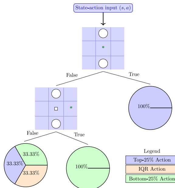
Fig. 7. Example multiclass classification tree for a handcrafted policy for Tic-Tac-Toe, modelled as a decision tree that takes state-action pairs (s, a) as inputs and produces a single classification for such a pair as output. This tree can recognise some winning actions (assuming this is a policy for the white player), classifying those actions as being likely top-25% actions. It can also recognise some cases where winning actions are possible but not picked (actions placing next to an empty cell in between two white pieces), and classifies those as being likely bottom-25% actions. Any other cases are classified as being equally likely to belong to any of the three possible classes.
