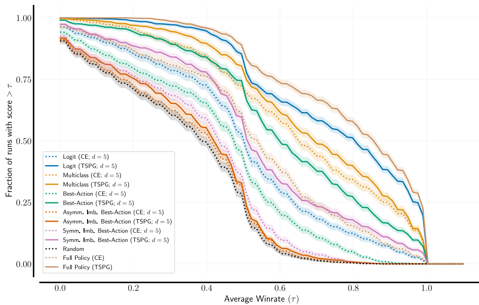
Fig. 12. Performance profiles summarising the performance of several agents (only displaying results for decision trees with depth limits of d = 5 ) across 30 different games. Performance is measured by the win rate averaged over all possible opponents (all other agents, including trees with depth limits d \neq 5 ).
