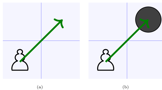
Fig. 3. Two example features that may or may not be equivalent depending on the game they are used in. Both encode, for grids of square cells, a diagonal move by a white pawn, but (b) has the additional restriction that the destination must be occupied by a black piece (of any type, indicated by a circle).
