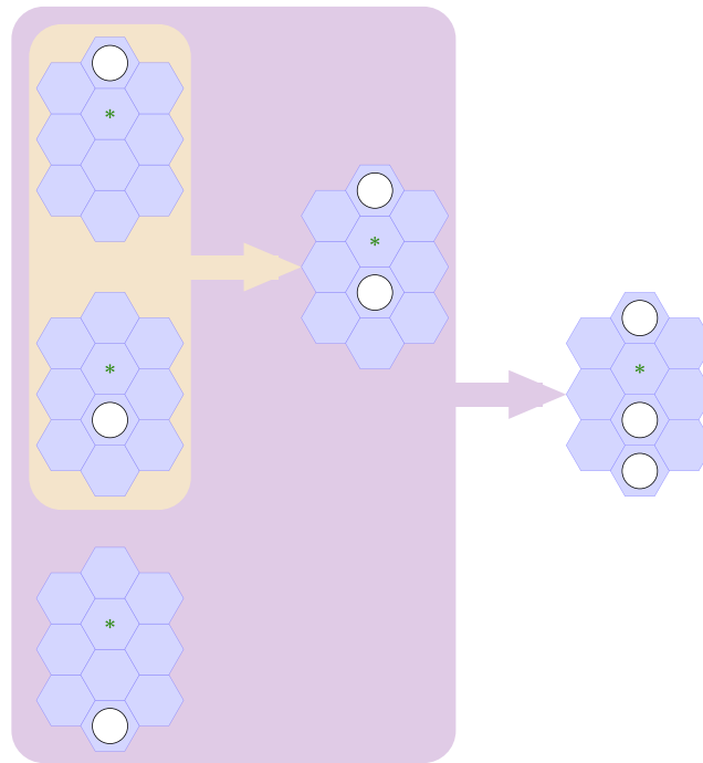
Fig. 2. Example of how new features are generated by combining instances of existing features. On the left-hand side, we start with three instances of atomic features. The top and middle instances are first combined into a new feature that matches actions that place a stone in between two white stones. This more complex feature is subsequently combined again with another feature, finally resulting in a feature that matches actions that complete or break a line of four white stones.
