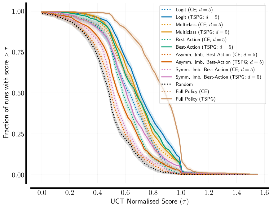
Fig. 10. Performance profiles [43] for several agents, summarising performance across all 13 small games. Performance is measured by UCT-normalised scores \tau , which are win percentages that have been linearly rescaled on a per-game, per-opponent basis, with the performance of UCT always being equal to 1.0.
