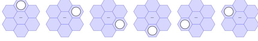
Figure 15: Six different instantiations, each with the same position (centre of the depicted area) as anchor, of a single feature that requires the anchor to be empty (indicated by “-”), and an adjacent position to contain a white stone. This means that every instantiation is a conjunction of two conditions, where the condition for the empty position is identical for each of the instantiations. The feature is a disjunction of these six conjunctions.
