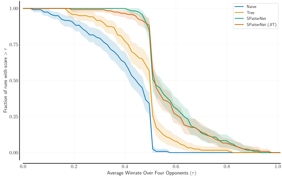
Figure 19: Performance profiles (Agarwal et al., 2021) for MCTS agents biased by trained features, with different approaches for evaluating features.
