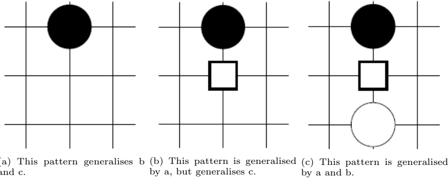
Figure 14: Three example patterns for Go in 3 \times 3 windows. Small squares denote positions that must be empty for the pattern to match, whereas any other empty positions are wildcard positions, the contents of which are irrelevant to pattern matching.
