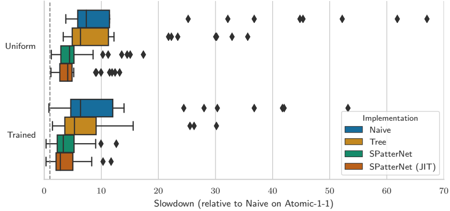
Figure 18: Boxplots summarising slowdowns of several feature evaluation implementations on large, trained feature sets; once where actions are sampled uniformly at random, and once where actions are sampled according to a trained policy. Every boxplot summarises 33 data points, from 33 different games. Lower slowdown values are better (with values < 1 being speedups—the dashed vertical line indicates this point).
