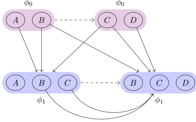
Figure 16: A network representation of features, feature instantiations, and propositions. Circles represent propositions, labelled with letters A, B, C, D . Coloured boxes represent feature instantiations—conjunctions of the propositions they surround. Instantiations are labelled and coloured according to the feature they represent. In this example, there are two features— \phi_0 and \phi_1 —with two instantiations each. A solid arrow from a proposition to an instantiation indicates that, if the proposition evaluates to false, the instantiation it points to is also disproven (in addition to the instantiation that the proposition is a part of itself). A dashed arrow from an instantiation f to another instantiation f' indicates that, if f is active, f' no longer needs to be evaluated.
