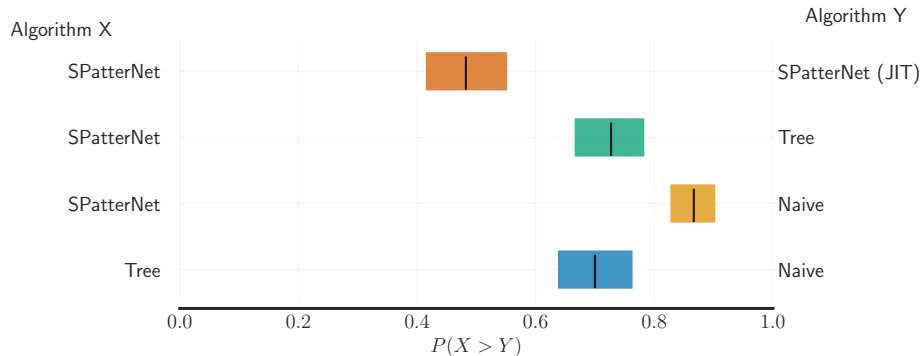
Figure 20: Pairwise probabilities of improvement (Agarwal et al., 2021) for algorithms on the left-hand side to outperform algorithms on the right-hand side.
